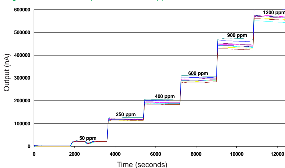
Figure 4 NO-B1 Response to 1,200ppm NO
