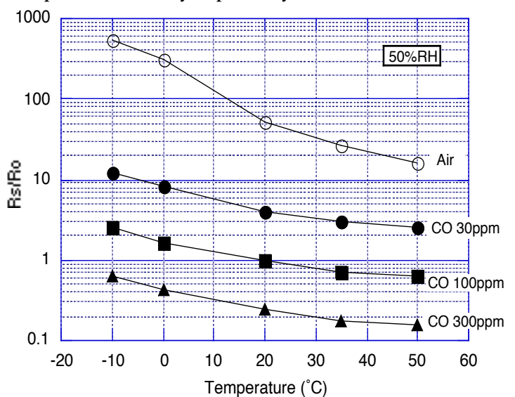
Temperature/Humidity Dependency:
